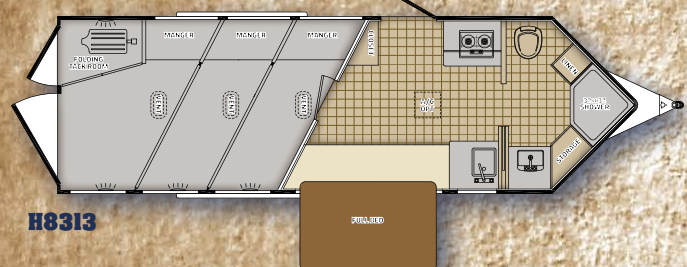
8' Wide HUT
